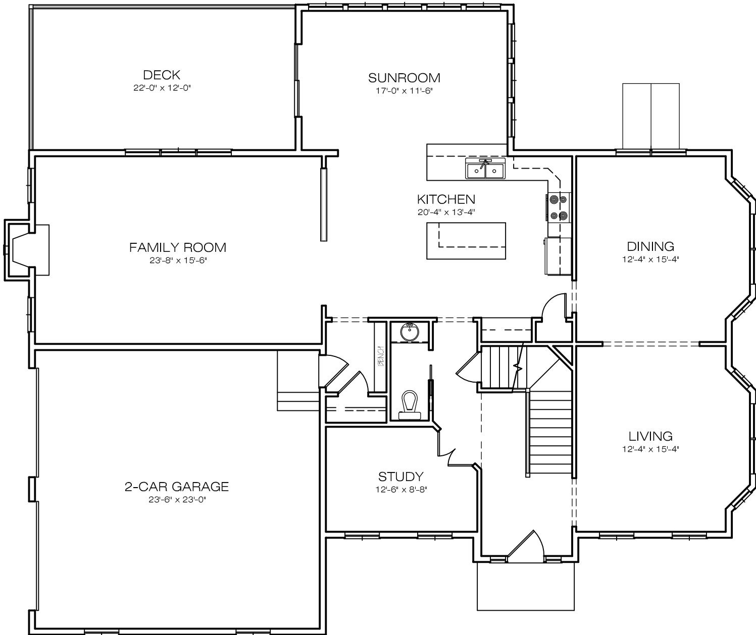
FIRST FLOOR PLAN PLAN # 3534
